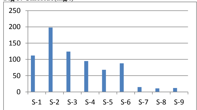
Fig 3. Chloride(mg/l)
