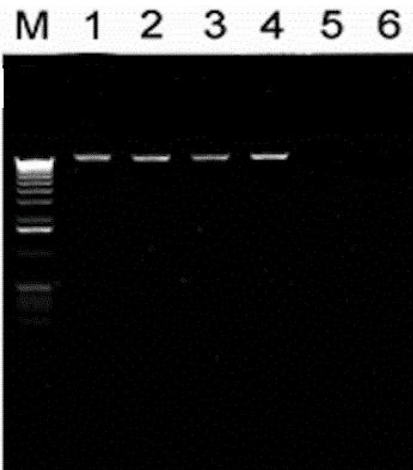
Figure 2. Agarose gel electrophoresis of various samples of P. monodon and A.indicus . Lanes are as follows; M lane- Marker, 1 lane- Peneaus monodon sample 1, 2 lane- Peneaus monodon sample 2, 3 lane- Acetes indicus sample 1, 4lane- Acetes indicus sample 2.
